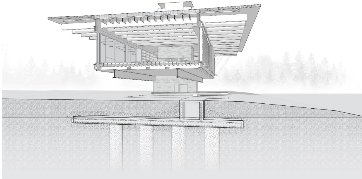
Project: Whistler Ski House, Olson Kundig Architects, Drawing by Nicholas Wong
