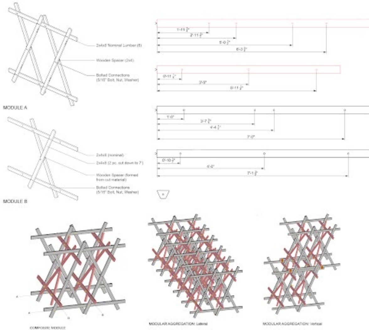
Shray Tripathi & Anishwar Tirapathur_ 2022 Carnival Entryway Pavilion Construction Drawings
